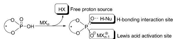
Scheme 1. Proposed cooperative catalytic system.
