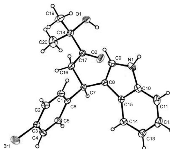
Figure 3. X-ray structure of 4ea .
