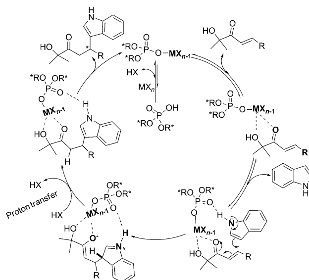
Scheme 2. Proposed proton-accelerated asymmetric Friedel–Crafts reaction process.
