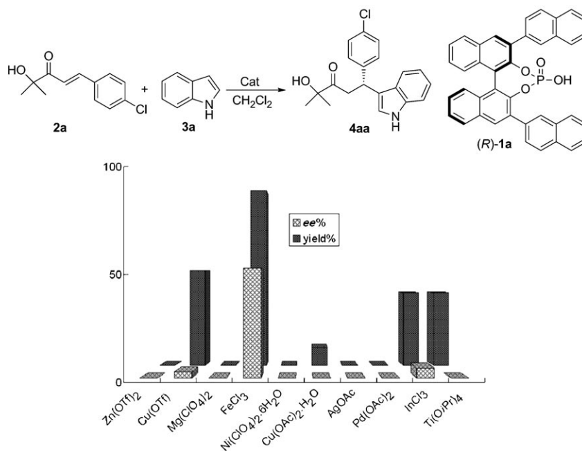
Figure 1. Screening of metal salts for the asymmetric Friedel–Crafts alkylation of indole with 1a as Brønsted acid.
