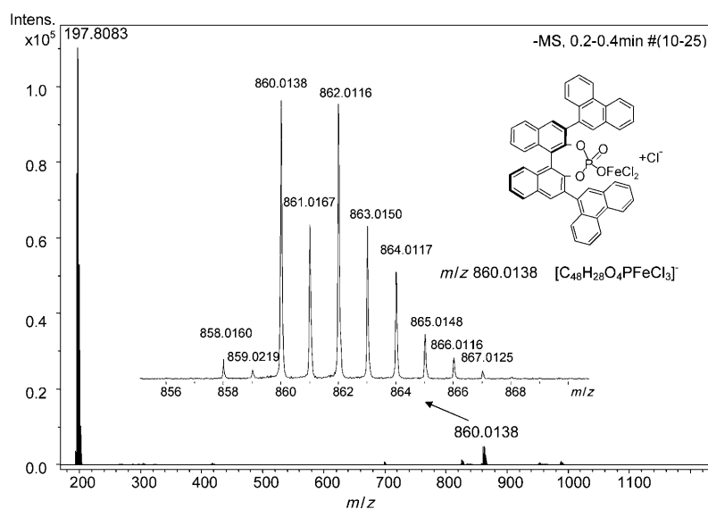
Figure 2. Confirmation of the existence of iron phosphate salt 1b /FeCl 3 .
